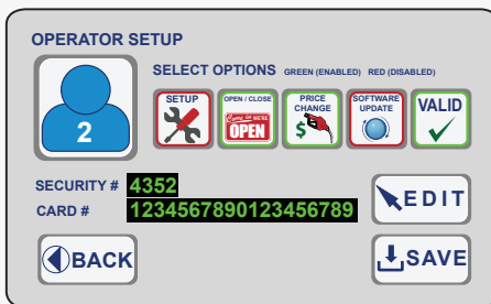
Operator Setup
